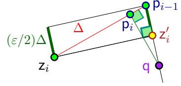
Figure 4.2: Worse case if extremal queries are approximate.
