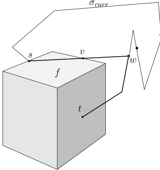
Figure 4: A single step of the main loop of PROJECT-PATH; \sigma_{curr} crosses H_f at three marked points, the last of which is w .
