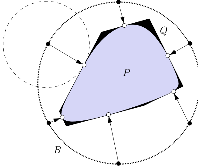
Figure 2: Approximating a convex shape using Dudley proof
