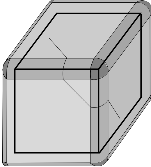
Figure 1: A cube P and the inflated set P_r
