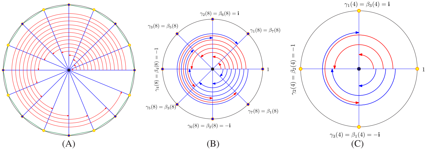
Figure 26.2: (A) The 16 roots of unity. (B) The 8 roots of unity. (C) The 4 roots of unity.
